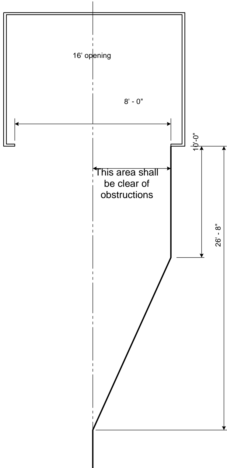
FIGURE 10: RESIDENTIAL GARAGE - TURNING CLEARANCE (FOR SINGLE FAMILY WELLINGS)
