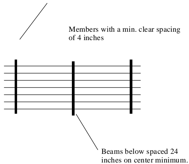
Diagram # 1 - Open egg-crate roof
